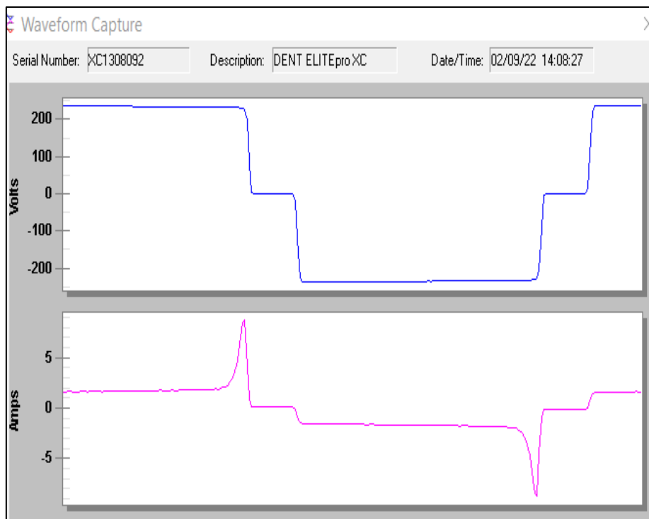
Figure 7: Voltage and Current Waveforms of the Inverter Output
