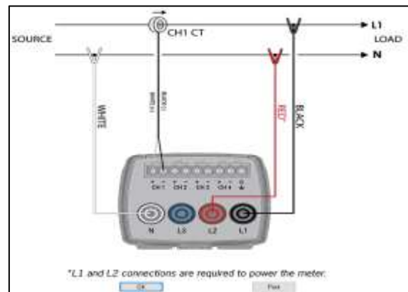
Figure 4: Typical Connection for the DENT Power Meter Used for the Harmonic Evaluation
